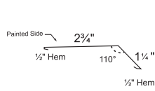
6. Gutter Guard
