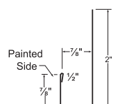
9. "J" Channel
