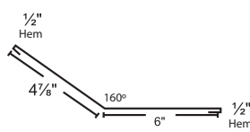
11A. Transition
