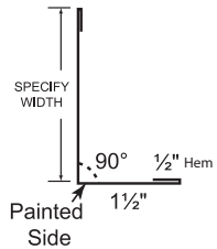
13. Fascia Trim
