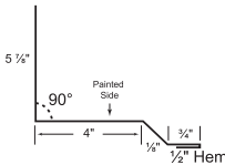
7. Sidewall Flashing
