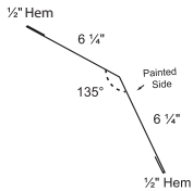
5A. Gambrel
