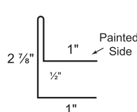
23. "F" Channel
